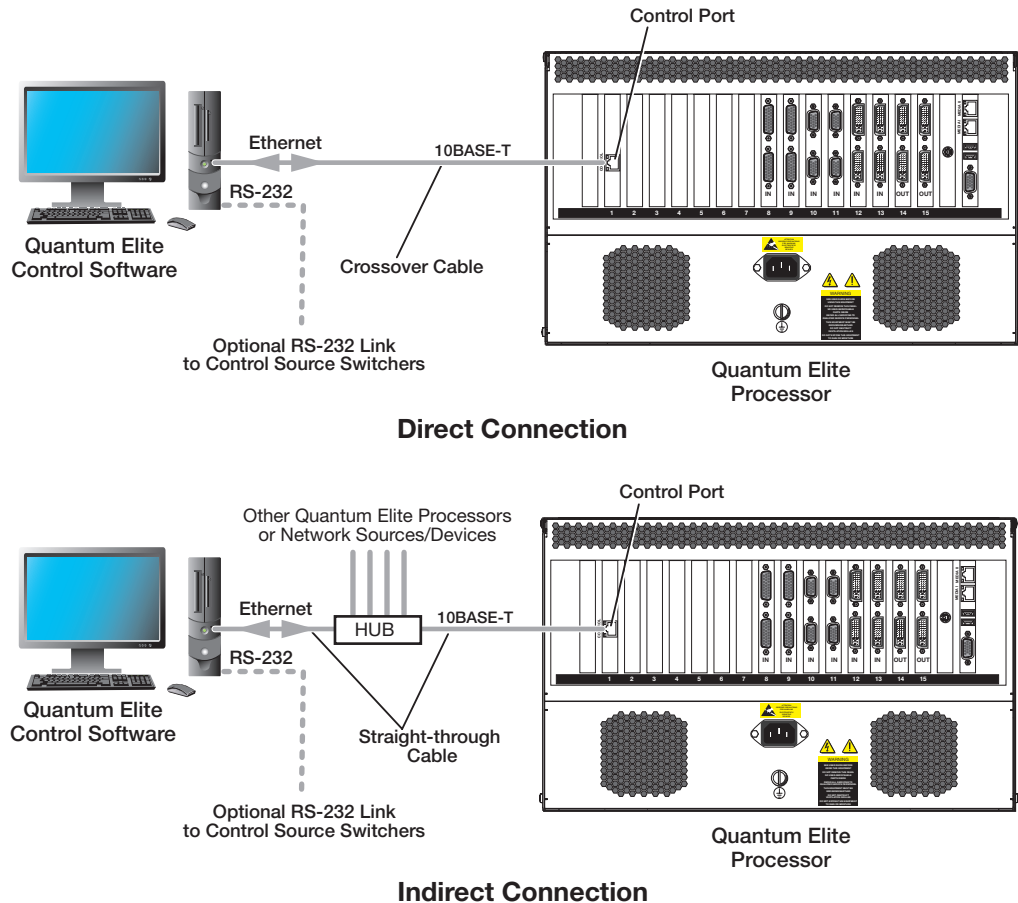
Figure 1. Methods of Connecting the Quantum Elite Control Software Computer to a Quantum Elite Processor
